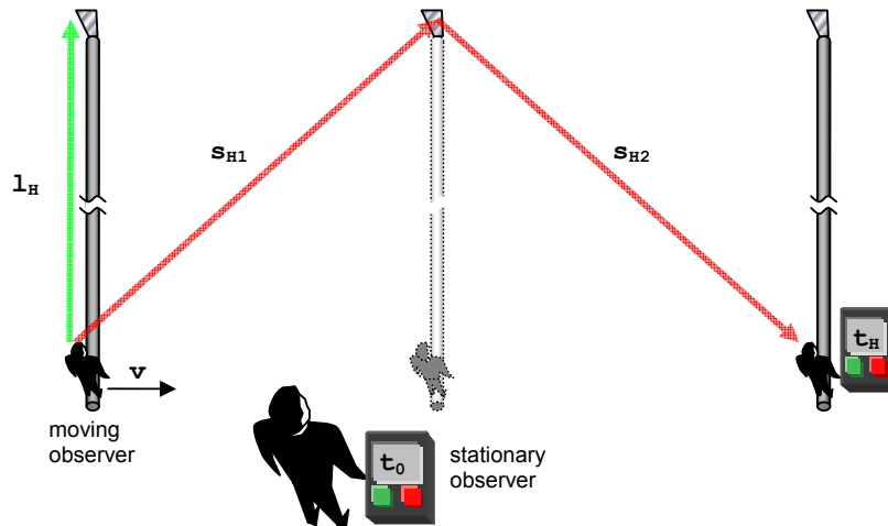
Fig. 1 Time dilatation is also valid upright to the direction of motion
