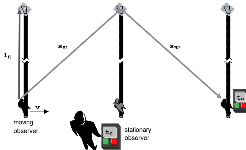
Fig. 1 Time dilation is also valid upright to the direction of motion
